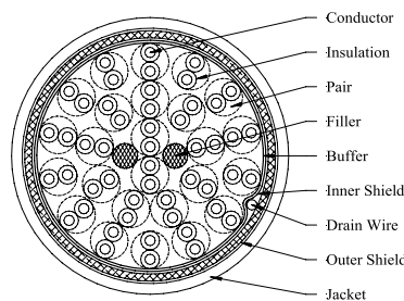
25 Pair 28 AWG Double Shielded Cable
