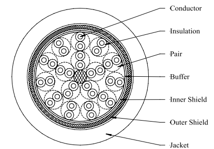
16 Pair 28 AWG Double Shielded Cable
