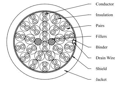
25 Pair 26 AWG STP Cable
