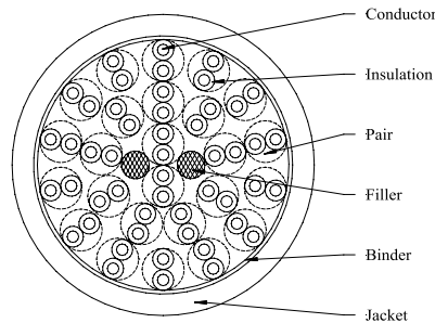
25 Pair 26 AWG UTP Cable
